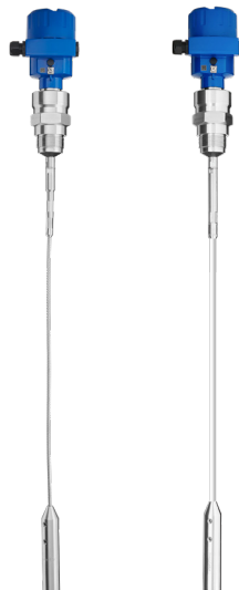
NG 3100 Rope version Customizable metal rope lengths
