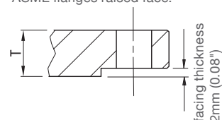
ASME flanges raised face:
